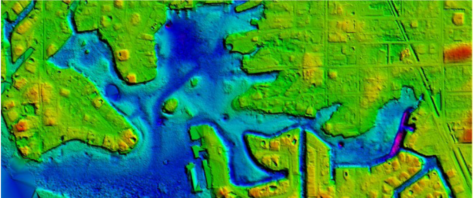
King's Bay Lidar Refinement Citrus County, FL
